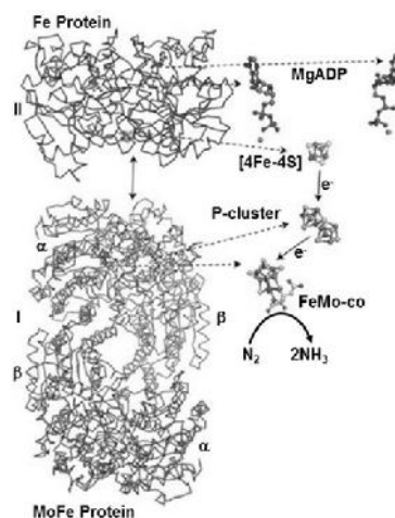
FIGURE 16.6 Structures of MoFe (Component I, nitrogenase) and Fe (Component II, nitrogenase reductase) proteins of nitrogenase, and electron flow through the two enzymes.
